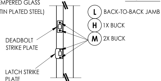
LATCH AND DEADBOLT DETAIL
