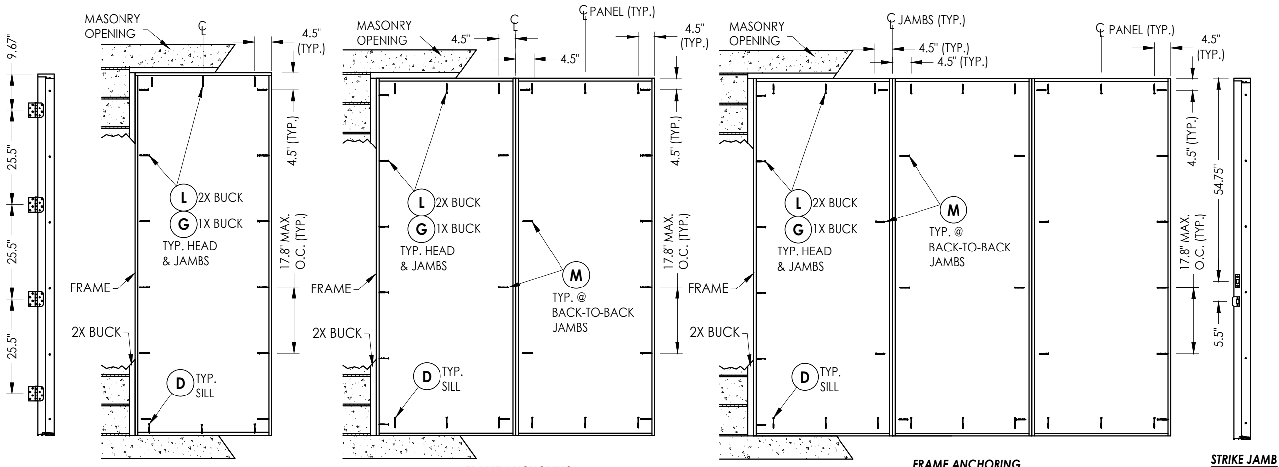
FRAME ANCHORING X
