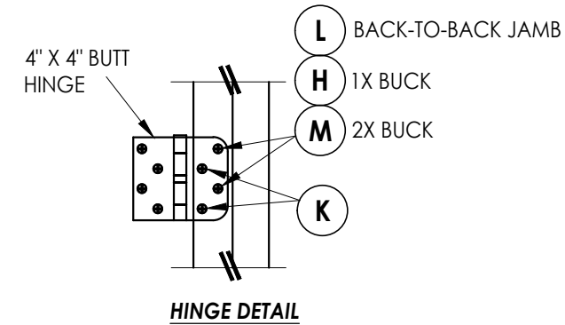
HINGE DETAIL
