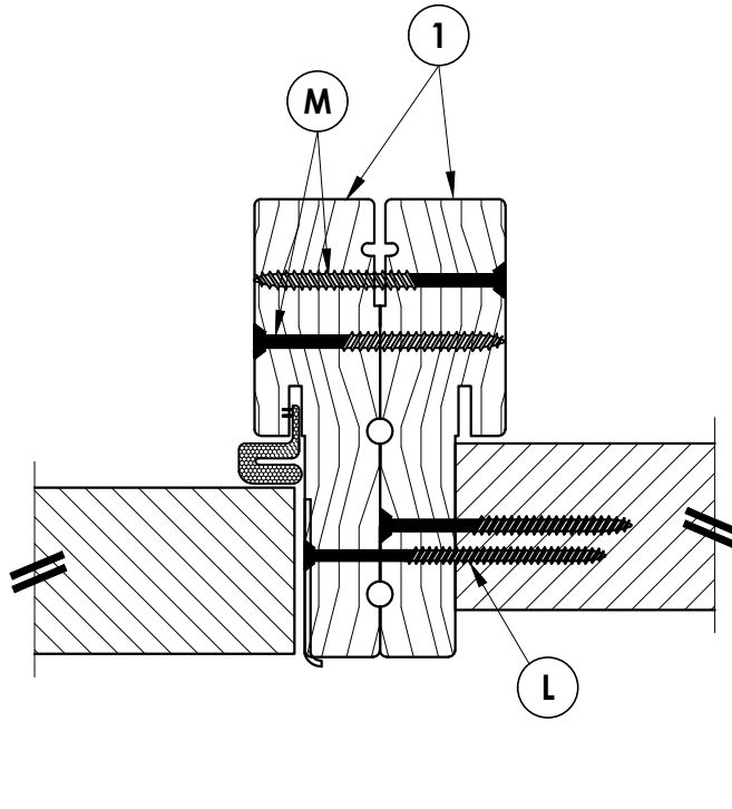
6 HORIZONTAL CROSS SECTION 2 @ BACK-TO-BACK JAMBS
