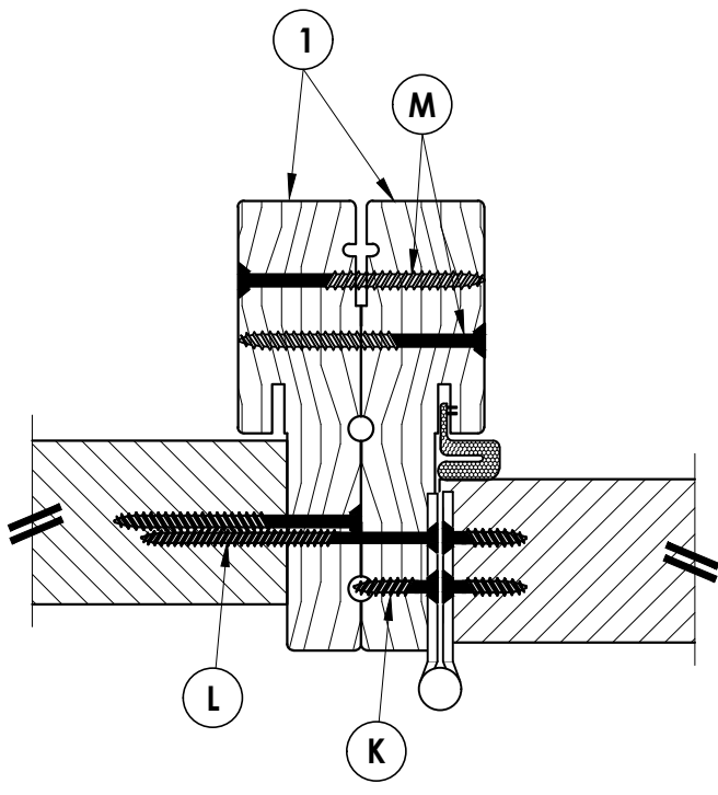
5 HORIZONTAL CROSS SECTION 2 @ BACK-TO-BACK JAMBS
